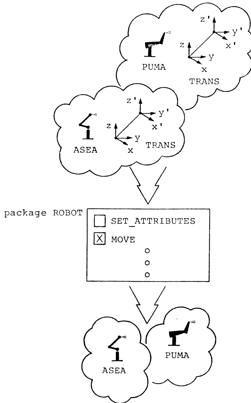
Figure 2. Data Abstraction.
