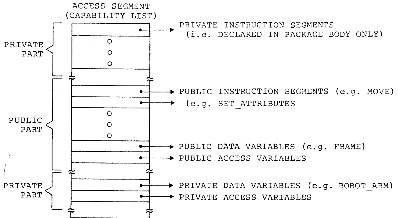
Figure 9. A Domain Object.
