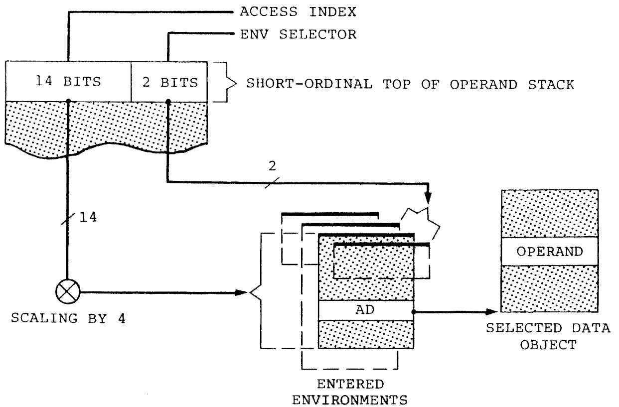
Figure 12. Stack Indirect Access Selection.
